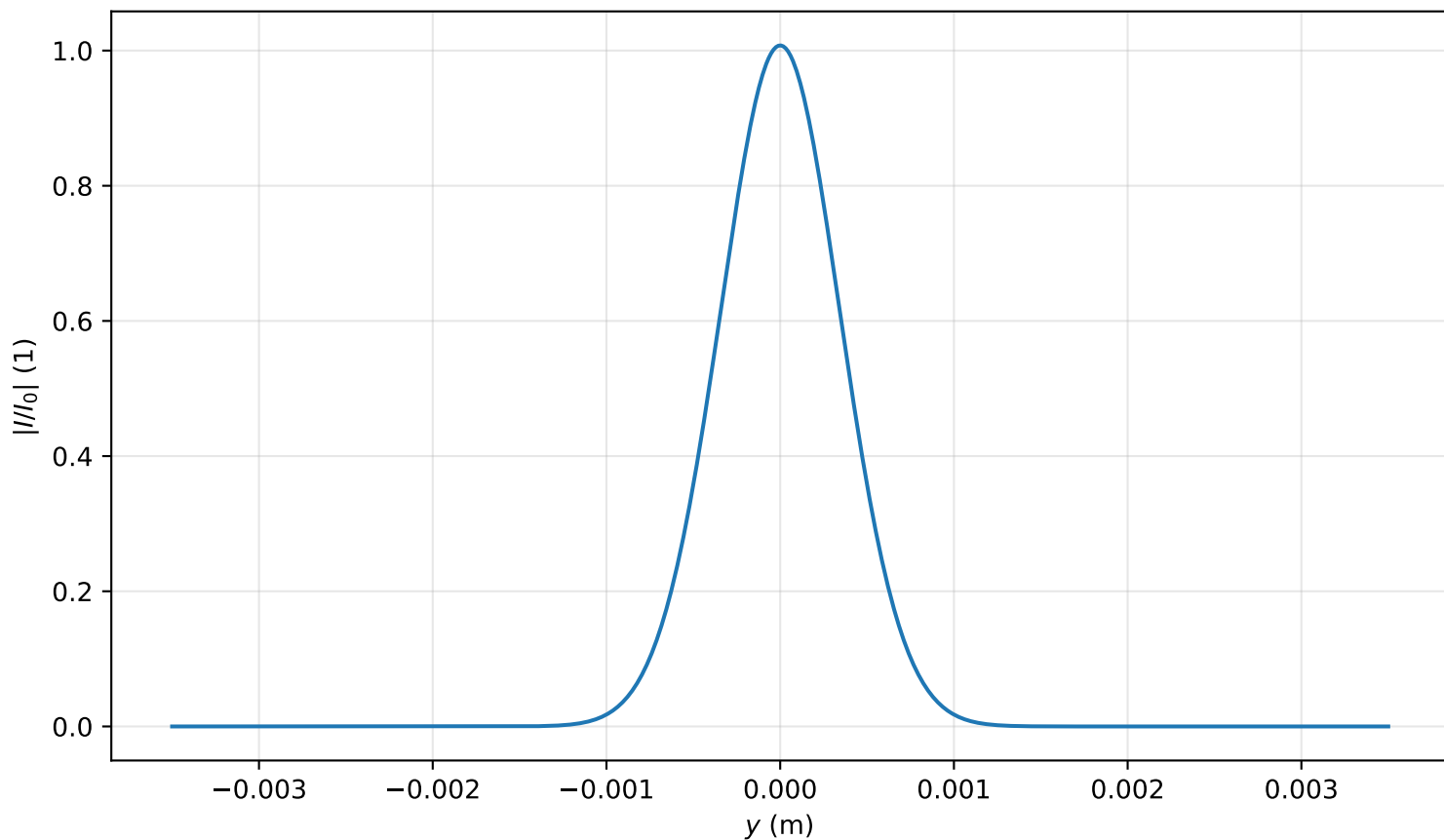
Intensity profile I(x=0, y, z=0.239)/I_0 , P_{in}=0.4P_{cr} , artificial time
